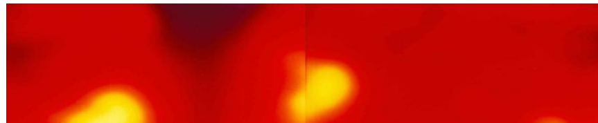
I. 6 months after solar eruption, stable geomagnetic condition (a negative node) 07.05.2004
