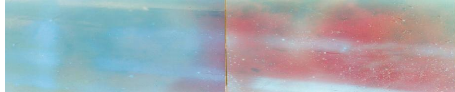
D. Traces of \alpha particles 17.07.2003
